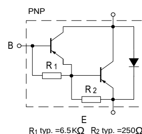
TO-126
