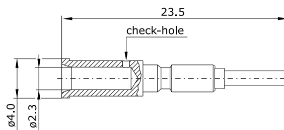
Main Dimensions contact pin
