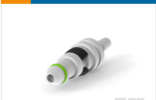
TE Part #1903100-2 PNEUMATIC CONN MALE CONTACTASSY DIA4 FKM
