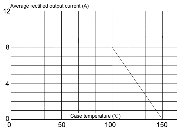
FIG.4: Average rectified output current derating curve
