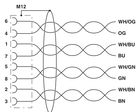
Contact assignment of the M12 socket
