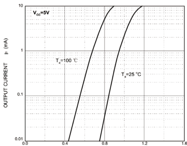
OFF Characteristics
