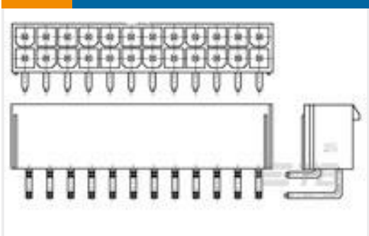
TE Part #1-1586041-4 14P VAL-U-LOK R/A HDR V2
