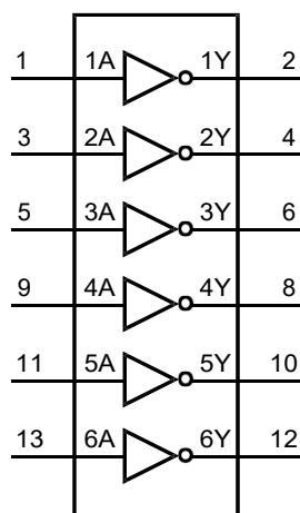
Figure 1. Logic symbol
