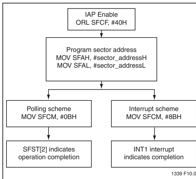
FIGURE 4-3: Sector-Erase
