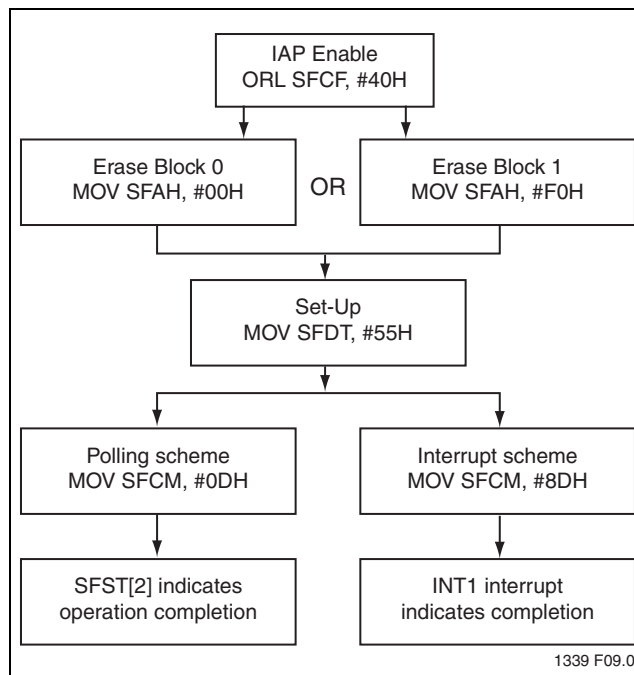
FIGURE 4-2: Block-Erase
