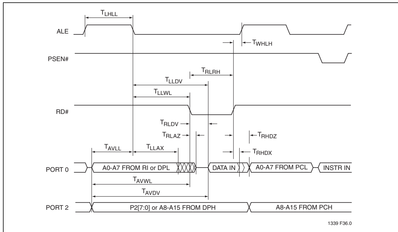
FIGURE 14-3: External Data Memory Read Cycle
