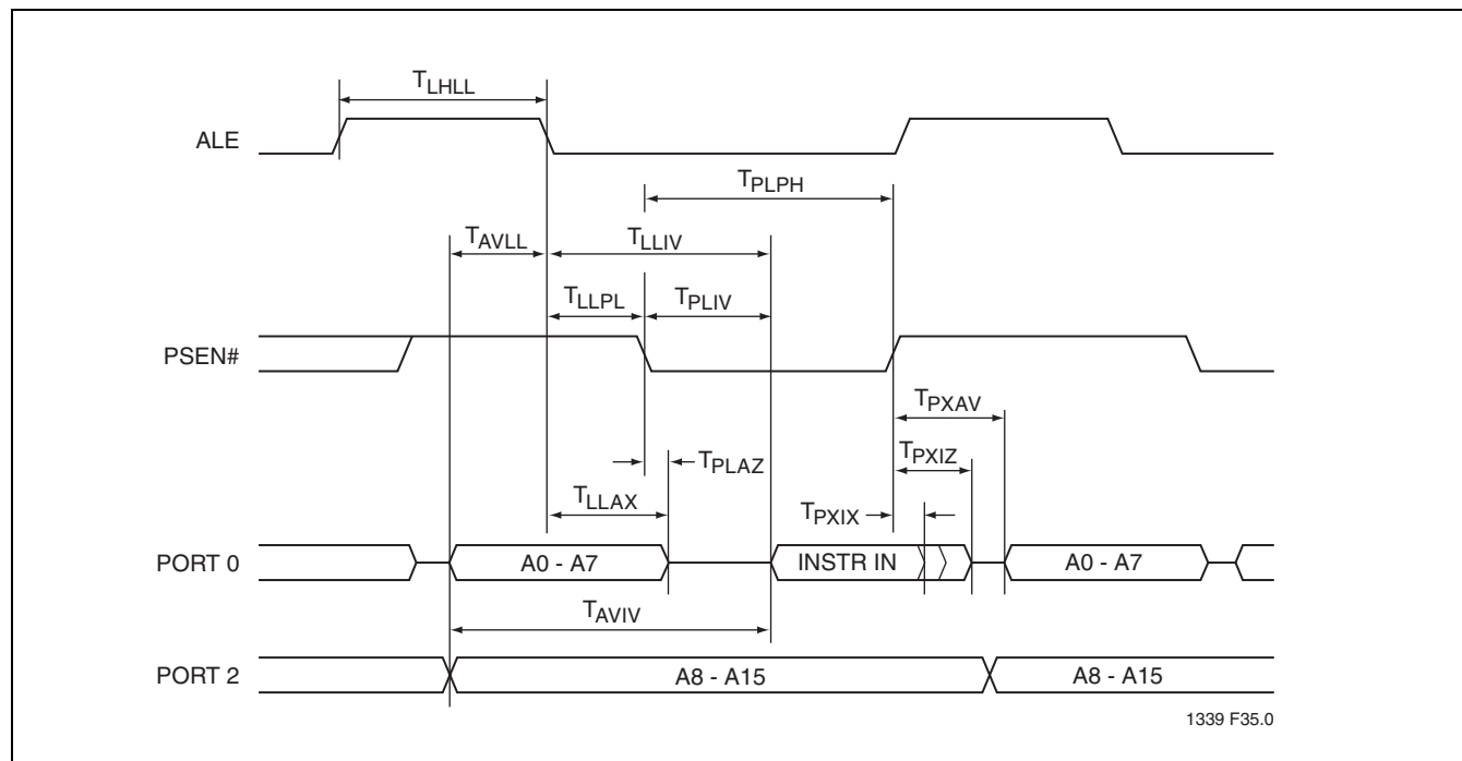
FIGURE 14-2: External Program Memory Read Cycle
