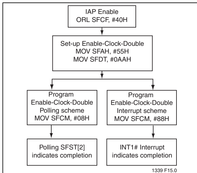
FIGURE 4-8: Enable-Clock-Double
