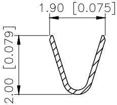
SECTION:A-A SCALE:1:1
