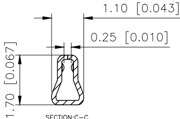
SECTION:C-C SCALE:1:1
