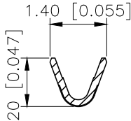
SECTION:B-B SCALE:1:1
