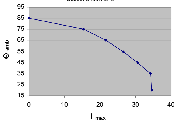
Max. allowable ambient Temp. at specific current (rms) B25667C4337A375
