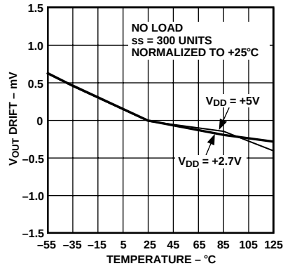
Figure 14. Zero-Scale Voltage Drift vs. Temperature
