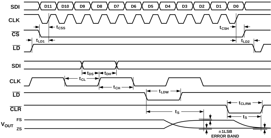
Figure 3. Timing Diagram
