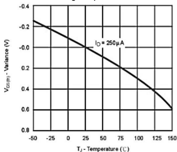
Fig.5 Threshold Voltage
