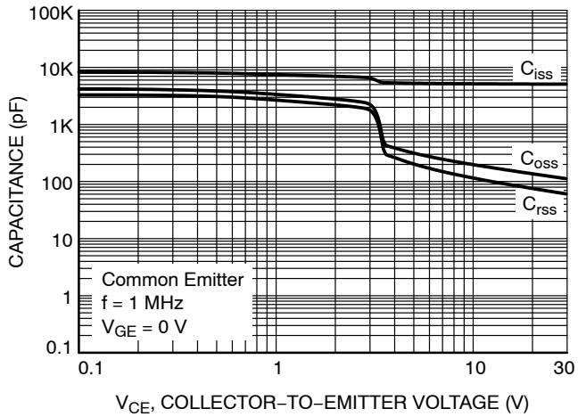
Figure 6. Capacitances Characteristics
