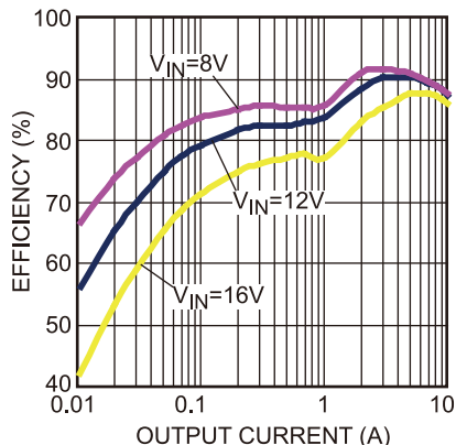
Figure 34 — Efficiency Curve
