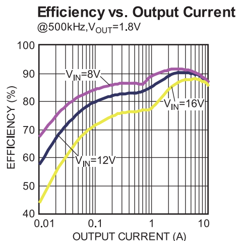
Figure 40 — Efficiency Curve
