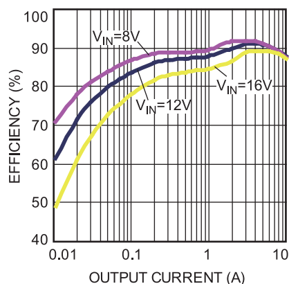
Figure 38 — Efficiency Curve
