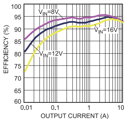
Figure 50 — Efficiency Curve
