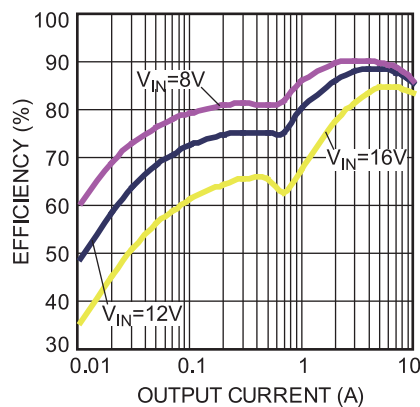
Figure 36 — Efficiency Curve
