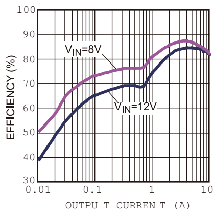
Figure 20 — Efficiency Curve
