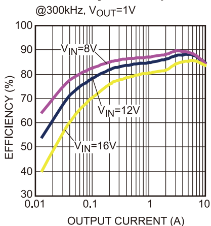
Figure 18 — Efficiency Curve
