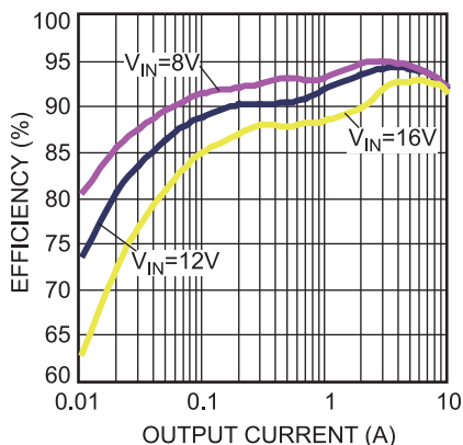
Figure 46 — Efficiency Curve
