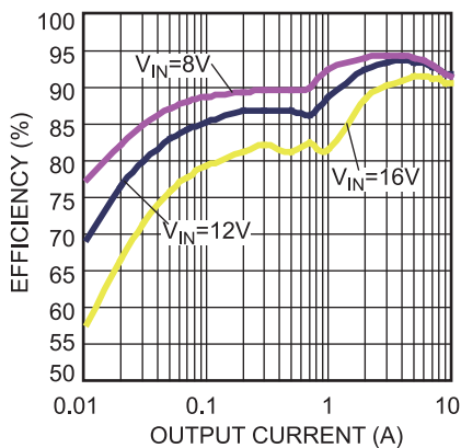
Figure 48 — Efficiency Curve
