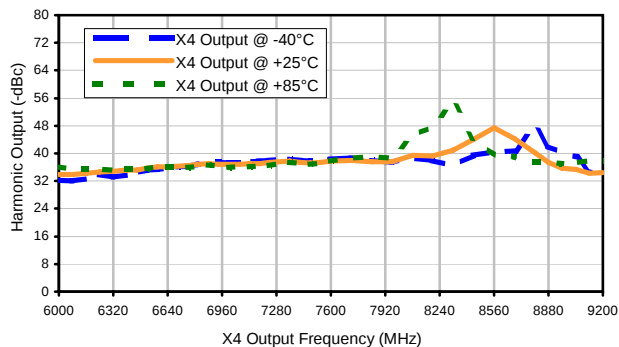
Harmonic X4 Output @ RF IN=13dBm
