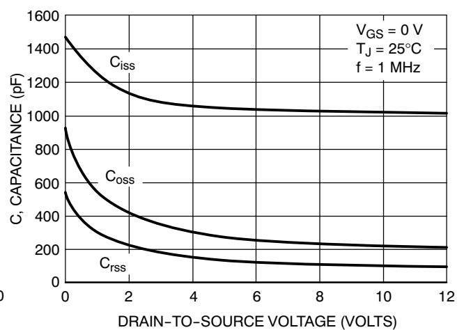
Figure 6. Capacitance Variation
