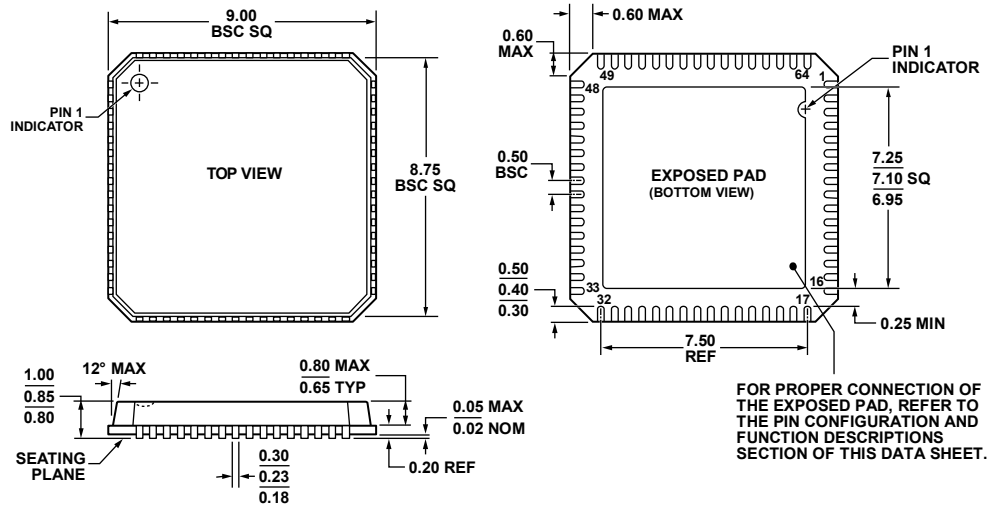
Figure 85. 64-Lead Lead Frame Chip Scale Package [LFCSP_VQ]
