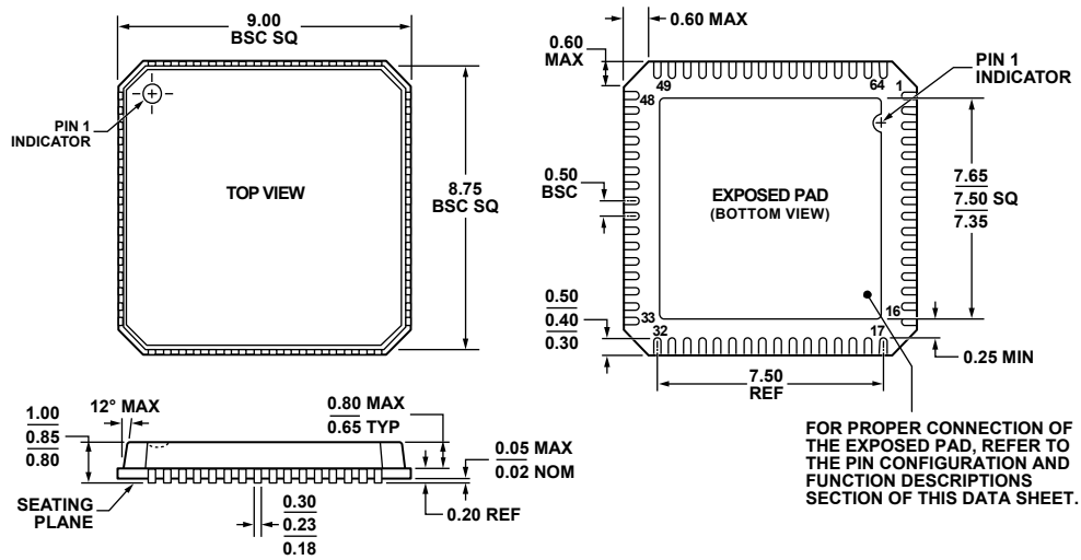
Figure 86. 64-Lead Lead Frame Chip Scale Package [LFCSP_VQ]
