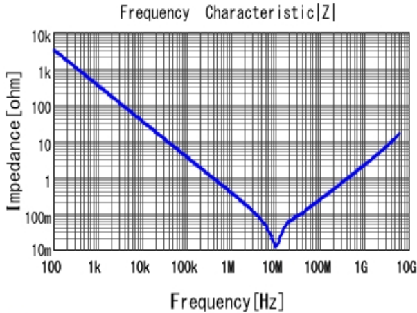
■ GRM188R61E684KA75 |Z| DC0V, 25degC
