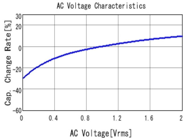
■ GRM188R61E684KA75 C-AC Voltage capchange, DC0V, 25.0d
