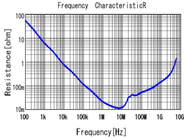
■ GRM188R61E684KA75 R DC0V, 25degC
