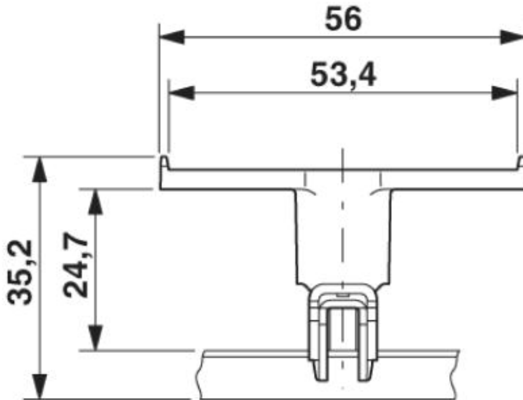
Dimensional drawing
