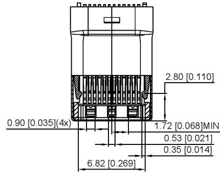
SECT B-B
