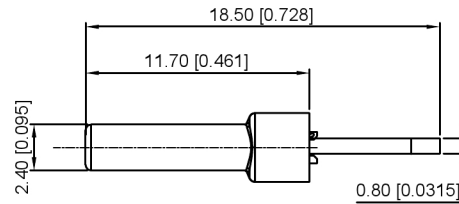
SECT B-B
