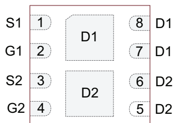
8-lead DFN (Dual Pad) (Top view)
