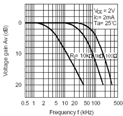
Fig.11 Frequency Response
