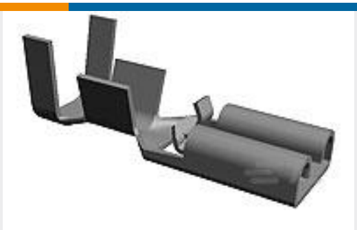
TE Part #1217096-2 PL 187 RECEPTACLE 18-14 AWG TPBR
