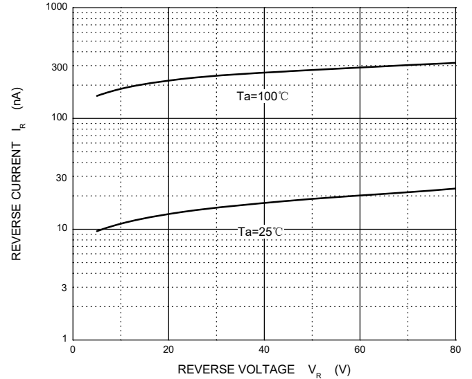
Reverse Characteristics
