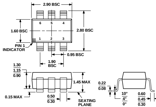
Figure 24. 6-Lead Small Outline Transistor Package [SOT-23] (RJ-6). Dimensions shown in millimeters.
