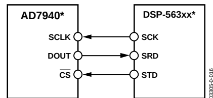
Figure 23. Interfacing to the DSP-563xx
