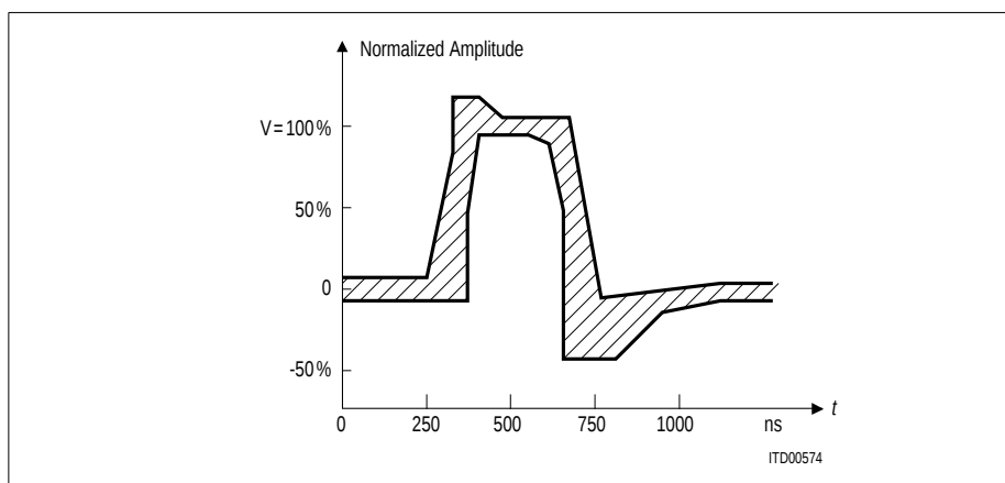
Figure 80 T1 Pulse Shape
