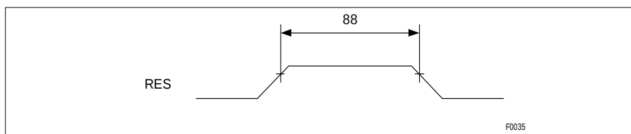
Figure 66 Reset Timing
