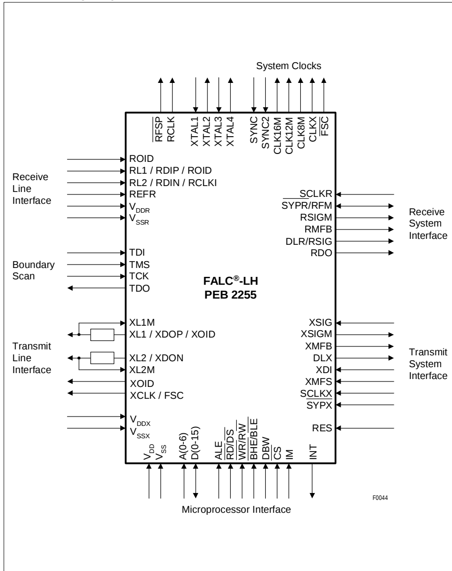
Figure 1 Logic Symbol
