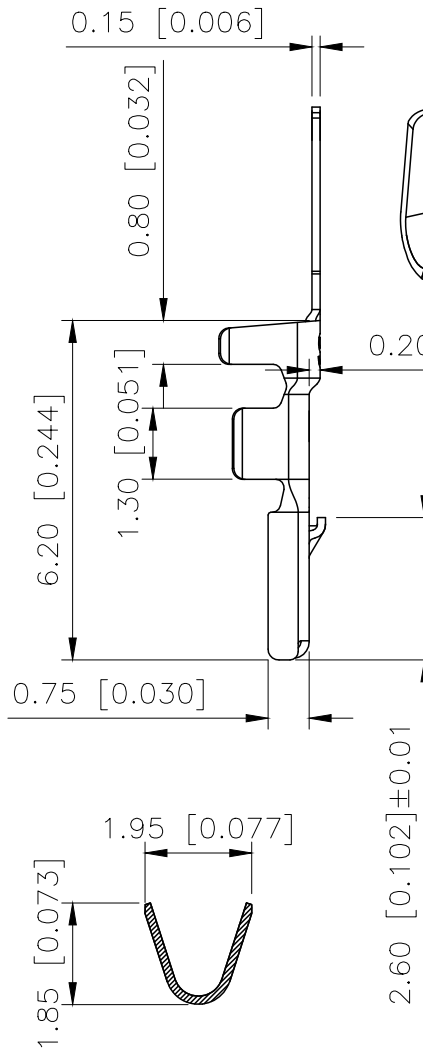
SECTION:B-B SCALE:1:1
