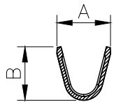
SECTION:A-A SCALE:1:1
