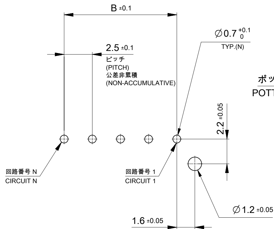
基板取付穴推奨寸法(マウント面) RECOMMENDED PCB HOLE DIMENSION (MOUNTING SIDE) ,(t=1.6)
