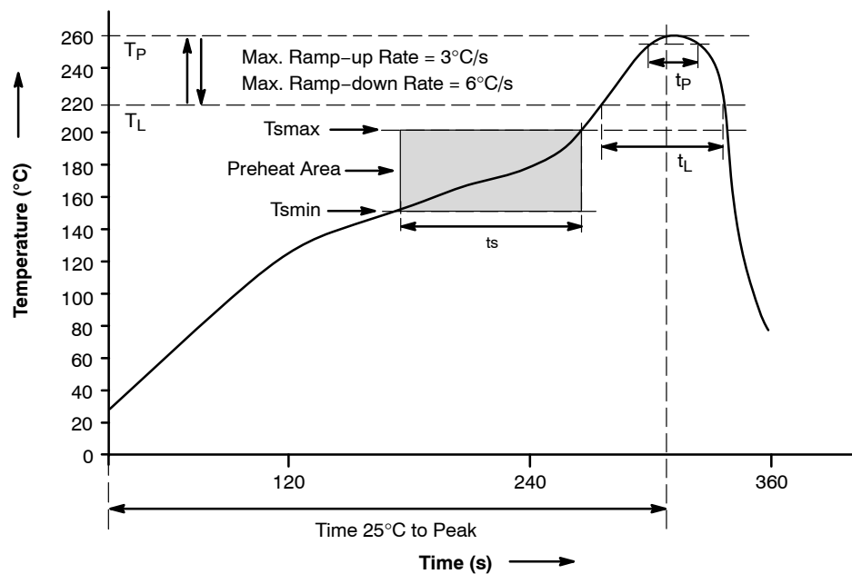
Figure 9. Reflow Profile
