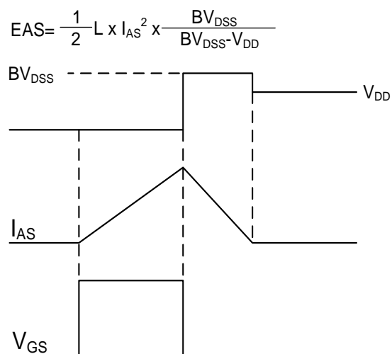
Fig.8 EAS Waveform
