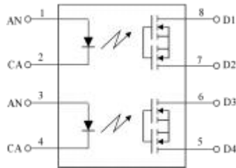
Pin Configuration
