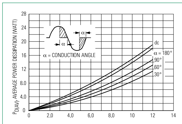
Figure 2. Power Dissipation
