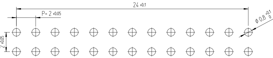
RECOMMENDED LAND PATTERN (FREE) (PCB THICKNESS t=1.6mm)
