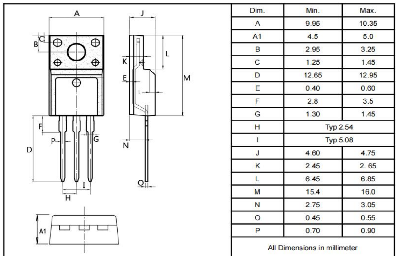
TO-220F
