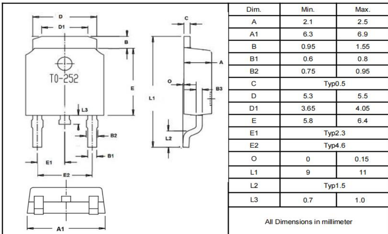
TO-252
