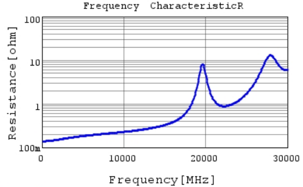
GJM0335C2A2R7WB01 R DCOV, 25degC
