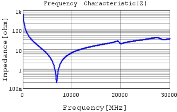
GJM0335C2A2R7WB01 |Z| DCOV, 25degC
