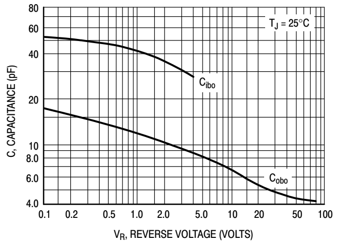
Figure 2. Capacitance
