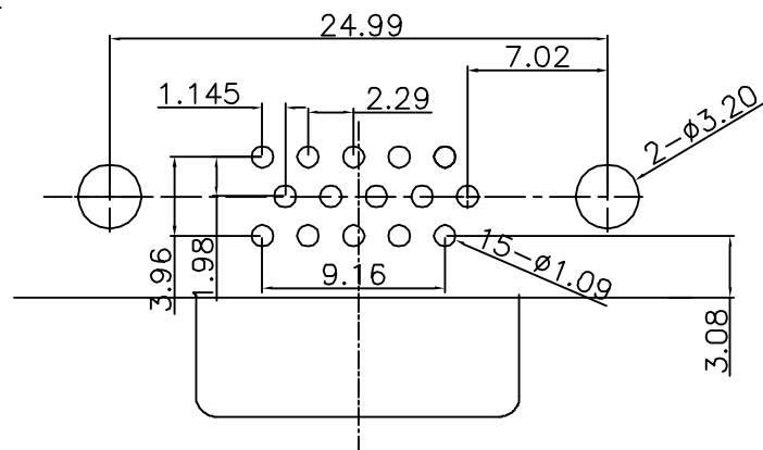
Recommended P.B.C Layout Top View
