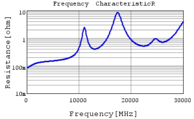
GJM0225C1E9R1WB01 R DCOV, 25degC
