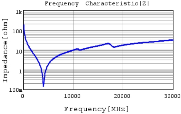
GJM0225C1E9R1WB01 |Z| DCOV, 25degC
