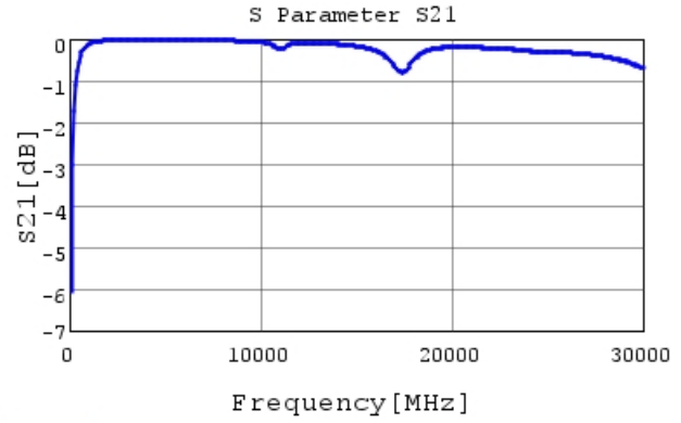
GJM0225C1E9R1WB01 S21 DCOV, 25degC
