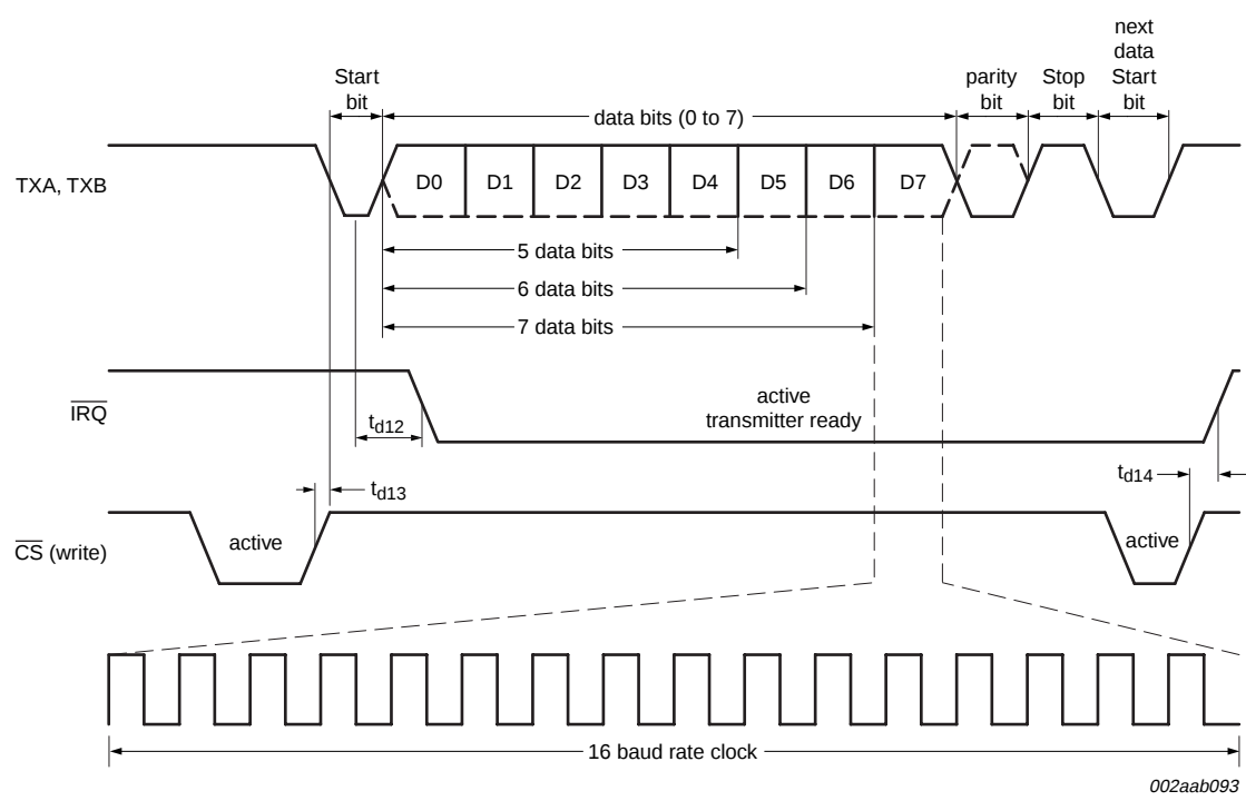
Fig 12. Transmit timing
