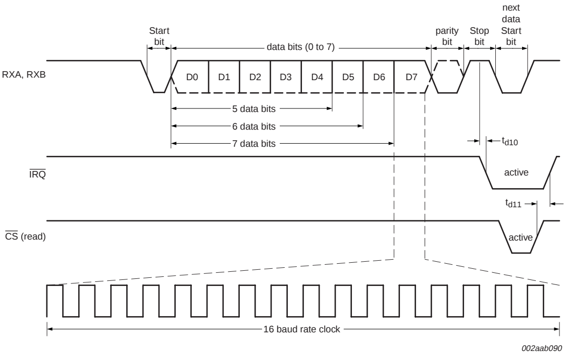
Fig 9. Receive timing
