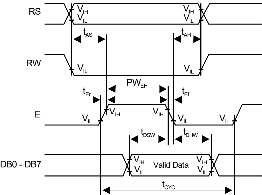
Fig.1 Write Operation Timing
