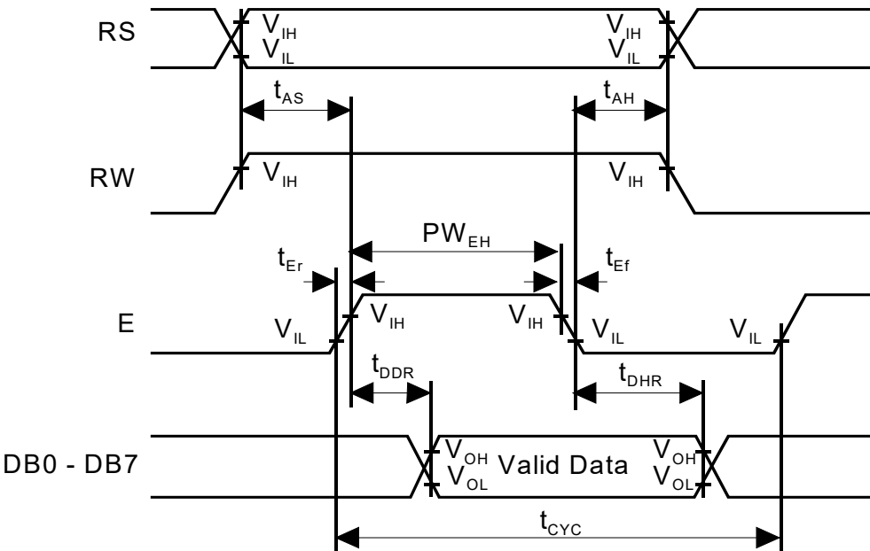
Fig.2 Read Operation Timing
