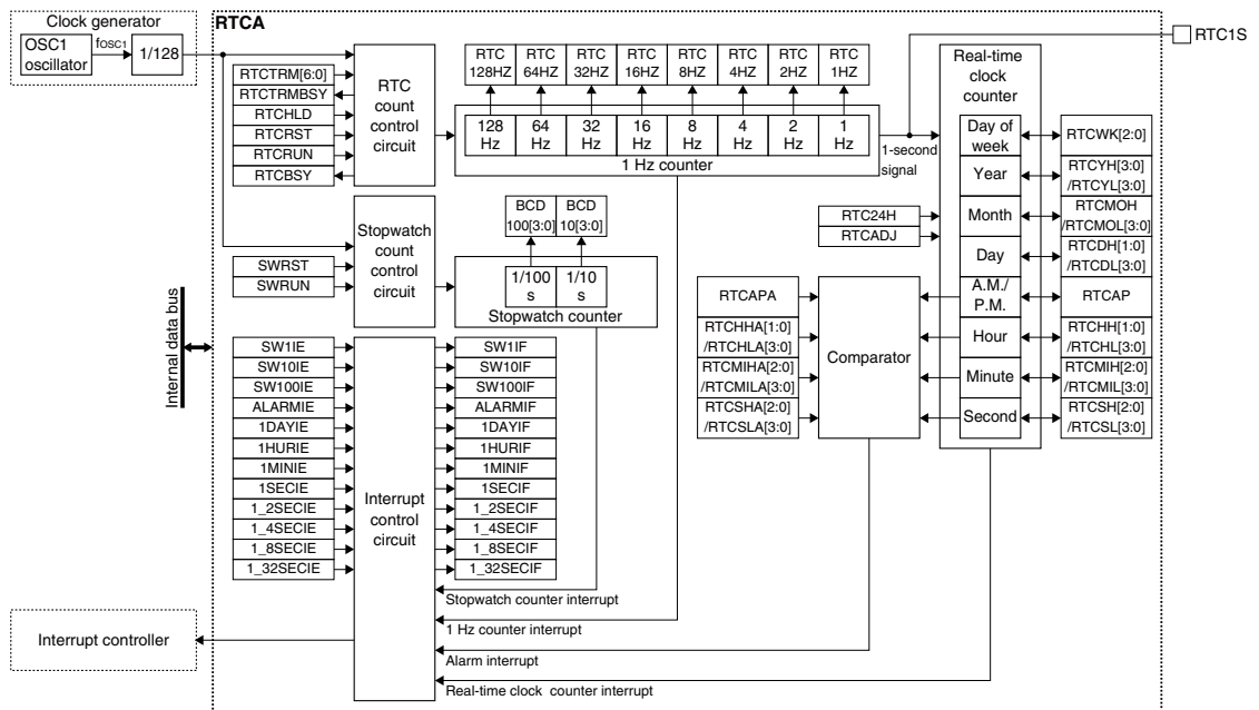
Figure 8.1.1 RTCA Configuration
