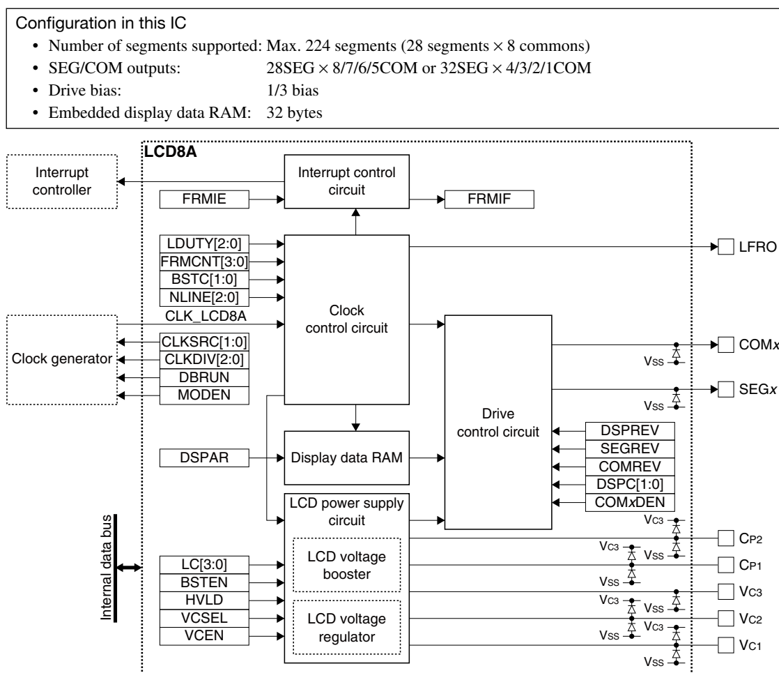
Figure 14.1.1 LCD8A Configuration
