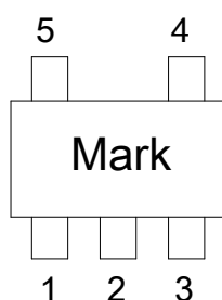
SOT-23-5L (Top View)
