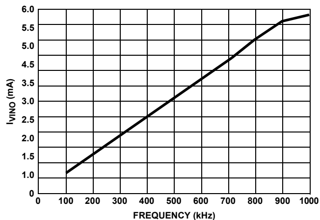
FIGURE 3. I_{VINO} vs FREQUENCY
