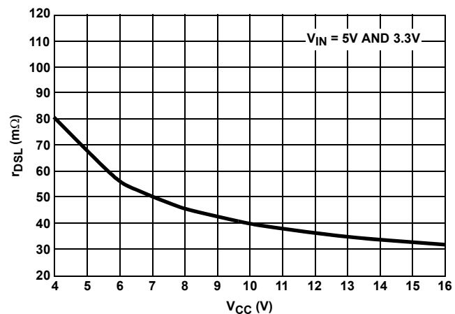
FIGURE 5. R_{DSL} vs V_{CC}
