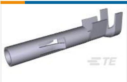
TE Part #350550-7 UMNL SOK 20-14 AU/BR L/P
