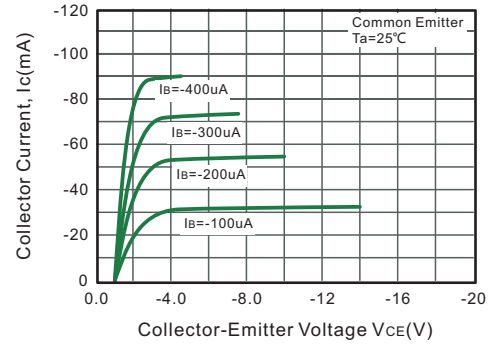
Fig.2 Static characteristics
