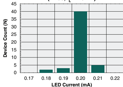
Typical I_F for Switch Operation (N=50, I_L=120\text{mA} )
