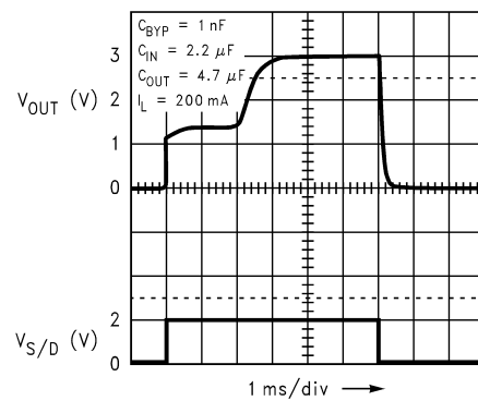
Turn-On Time (LP2988)
