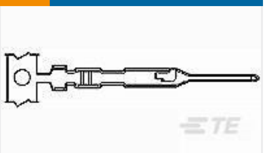
TE Part #5-104506-3 MTE PIN LP
