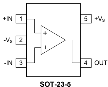
SGM8291BYN5G (TOP VIEW)
